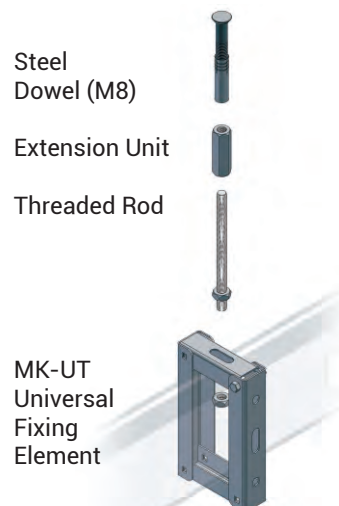
Roof Installation
