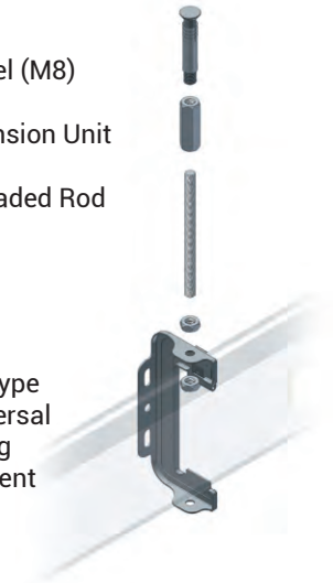
Roof Installation
